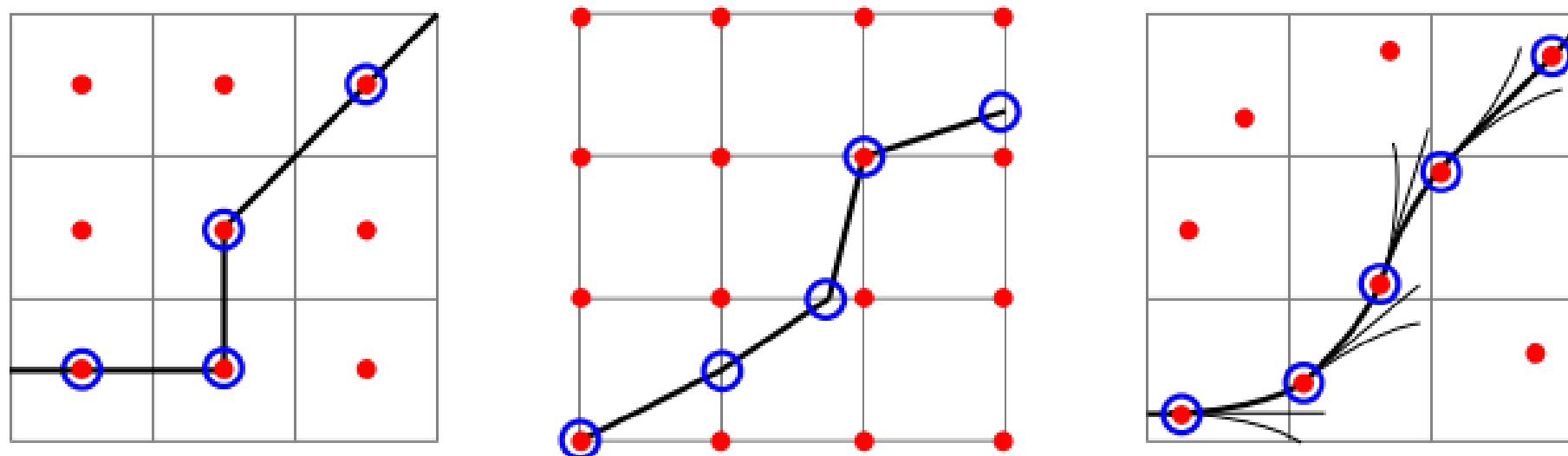
FIGURE 1: Comparison of search algorithms. Nodes are represented by the red dots. Left: A*, centre: D*, right: hybrid-state A*. [4]
